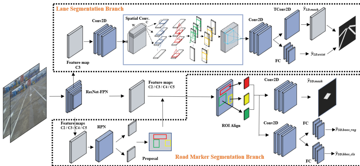
Fig. 2. LDS-Net architecture. It contains three modules: ResNet-FPN for multiscale feature extraction, a lane segmentation branch, and a road marker segmentation branch. Blue blocks denote network layers, while gray blocks denote features in embedding spaces (best viewed in color).
