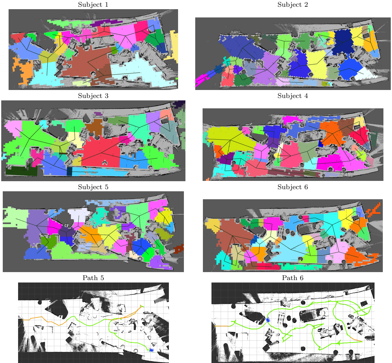
Fig. 16 Topological segmentation at the end of each subject’s trial and examples of different paths performed by subjects 5 and 6. Map size is in average 53 \times 23 \text{ m}^2 . Please refer to table 2 for statistical results. A sample dataset of the incremental mapping process is accessible at: http://www.ece.ust.hk/~eelium/mapping_bag_tunnel_subject1.bag (117MB)
