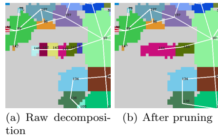
Fig. 11 Fusion of pruned regions applied to the sample map.
